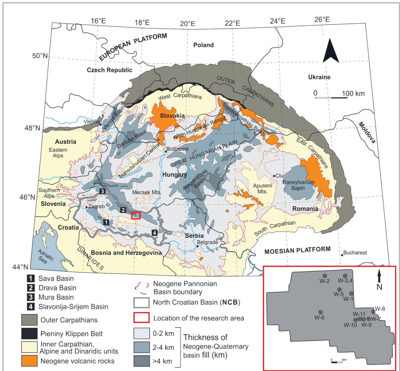
Figure 1. The Pannonian Basin System with the outline of the North Croatian Basin and the study area location. The red rectangle represents the extent of 3D seismic coverage of the “Donji Miholjac” 3D seismic block with the locations of 11 wells highlighted, enlarged in the inset at lower right corner (modified from Cvetković et al. (2019), after Dolton (2006) and Schmid et al. (2008)).
