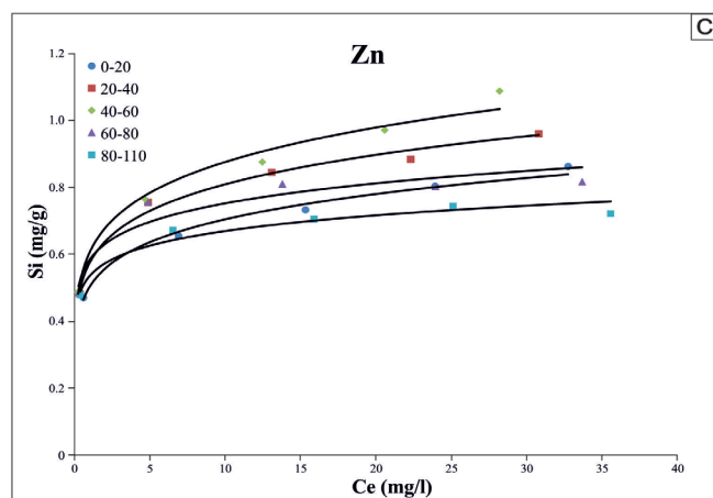
Figure 6. Freundlich sorption isotherms for Profile 3: a) Cu; (b) Cd; (c) Zn.
