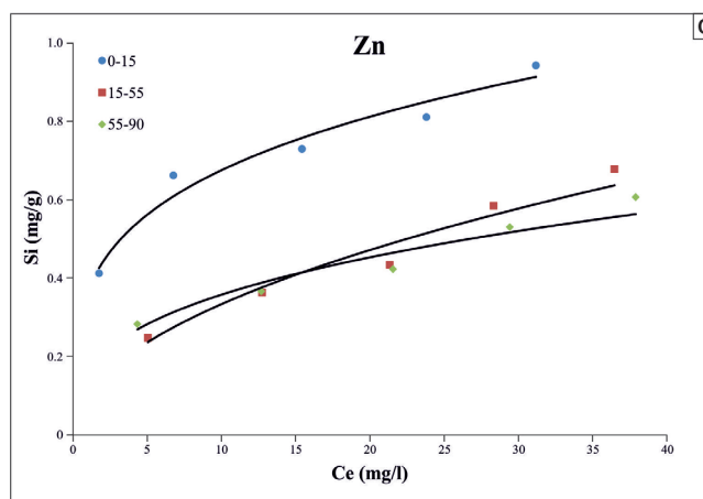
Figure 7. Freundlich sorption isotherms for Profile 4: a) Cu; (b) Cd; (c) Zn.
