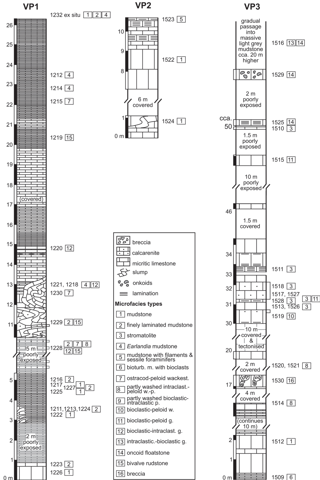
Figure 6. Sections of the Velika planina member.
