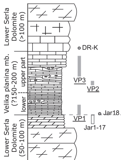
Figure 4. Schematic stratigraphic column with relative positions of samples and sections.
