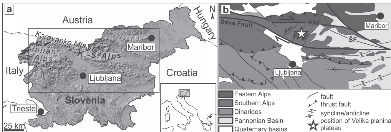
Figure 1. Geographical and structural position of the Velika planina plateau. a Map of Slovenia with the location of the Kamnik-Savinja Alps. The smaller rectangle shows the position of the inset in Figure 1b. Source: Digital elevation model with 5 x 5 m raster grid, DEM 5, 2006. Slovenia, Public Information of Slovenia, The Surveying and Mapping Authority of the Republic of Slovenia. b The tectonic structure of central and northern Slovenia. The position of the Velika planina plateau is indicated by a star symbol. PAF: Periadriatic Fault. ŠF: Šoštanj Fault. Modified after VRABEC & FODOR (2006).
