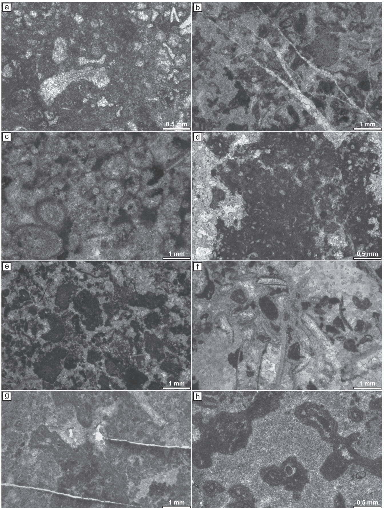
Figure 5. Microfacies of the Lower Serla Dolomite. a) Partly washed bioclastic wackestone. Thin section 1490. b) Partly washed intraclastic-bioclastic wackestone to packstone. Thin section 1496. c) Dolomitized dasycladacean (?) grainstone. Thin section 1486. d) Large microbialite intraclast within a microbial intraclastic rudstone. Thin section 1495. e) Intraclastic grainstone matrix of a microbial intraclastic rudstone. Thin section 1497. f) Dolomitized bivalve rudstone. Thin section 1493. g) Microbialite boundstone. Thin section 1501. h) Microbialite wackestone or bafflestone. Thin section 1488.
