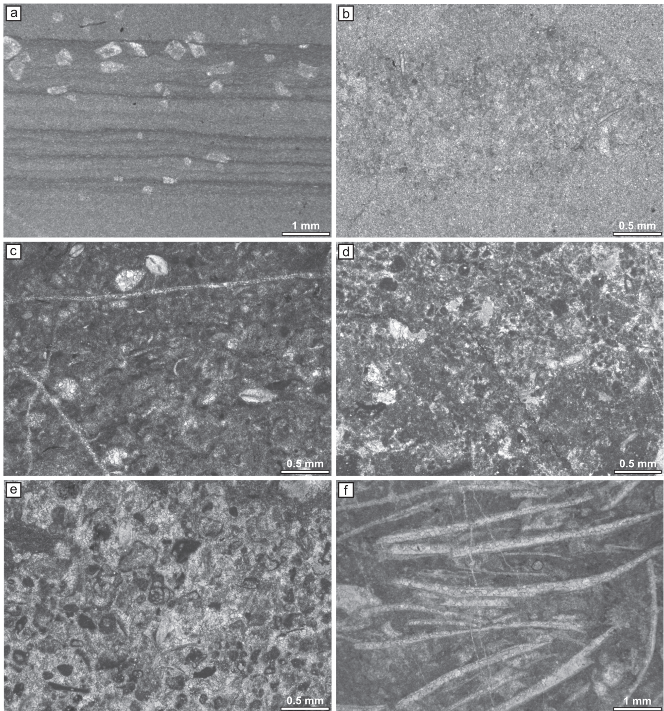
Figure 7. Microfacies of the Velika planina member, section VP1. a) Finely laminated mudstone. Note rhomboidal crystals of calcite. Thin section 1232b. b) Earlandia mudstone. Note the foraminifer Earlandia tintinniformis (Mišik) in the darker lamina. Thin section 1232c. c) Peloid wackestone with ostracods. Thin section 1230. d) Partly washed intraclastic-peloid wackestone to packstone. Thin section 1228d. e) Intraclastic-bioclastic grainstone. Note the foraminifer Glomospira sp. in the centre. Thin section 1228c. f) Bivalve floatstone. Thin section 1219.
