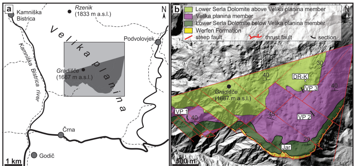
Figure 3. Geological map of part of the Velika planina plateau. a) Position of the studied area. b) Geological map and position of the sections.
