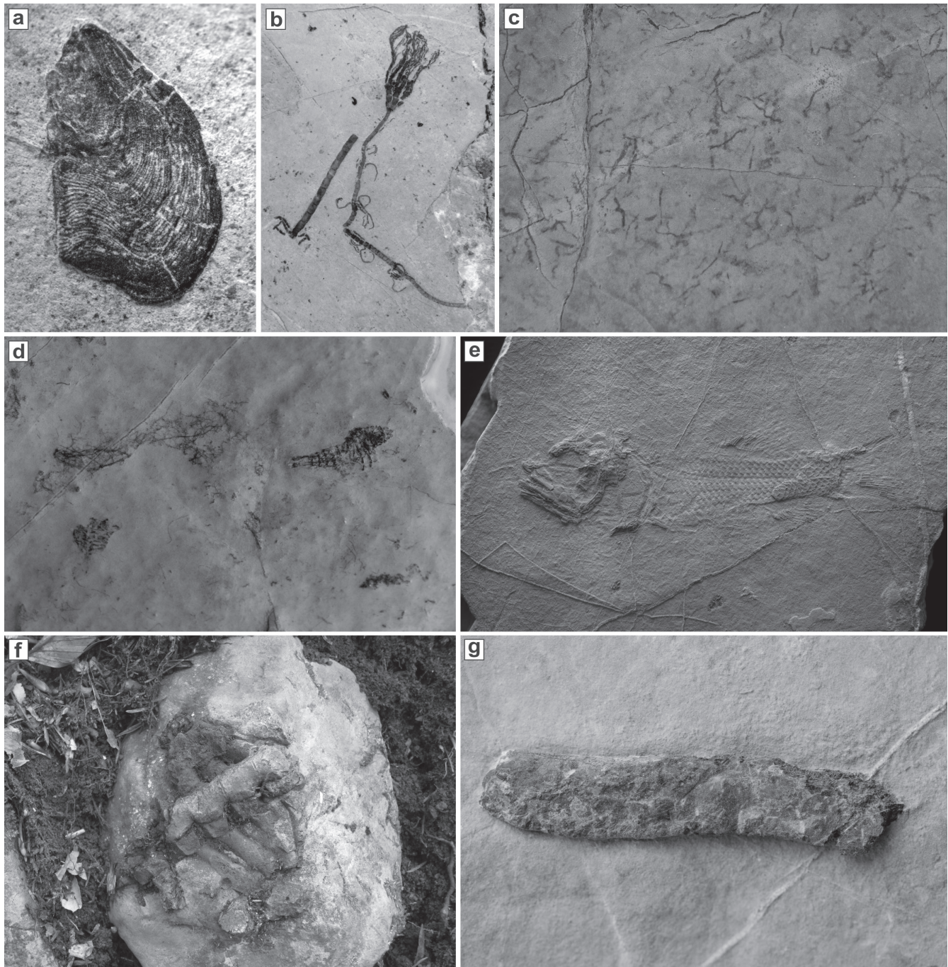
Figure 9. Fossils of the Velika planina member. a) A bivalve Bakevellia costata ; length 7 mm. b) An undescribed crinoid; length of the crown 9 mm. c) Chondrites ichnogenus; width of the photo is 4 mm. d) A mass mortality bed with arthropod remains and the trace fossil Chondrites ; length of the arthropod on the right is 5 mm. e) A fish of the genus Furo coated by ammonium chloride sublimate; length of the fish is 5 cm. f) A sacral region of a sauropterygian reptile of the order Nothosauroidea exposed on the site, length of the specimen is 9 cm. g) A coprolite; length is 5 cm. Image credit: (A, B, E): Jure Žalohar Tomaž Hitij; (C, D, F): Tomaž Hitij.
