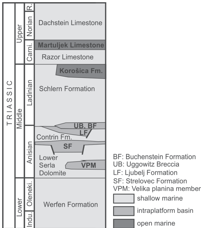
Figure 2. Stratigraphic column of the Triassic in the Kamnik-Savinja Alps. Modified after ŽALOHAR & CELARC (2010).
