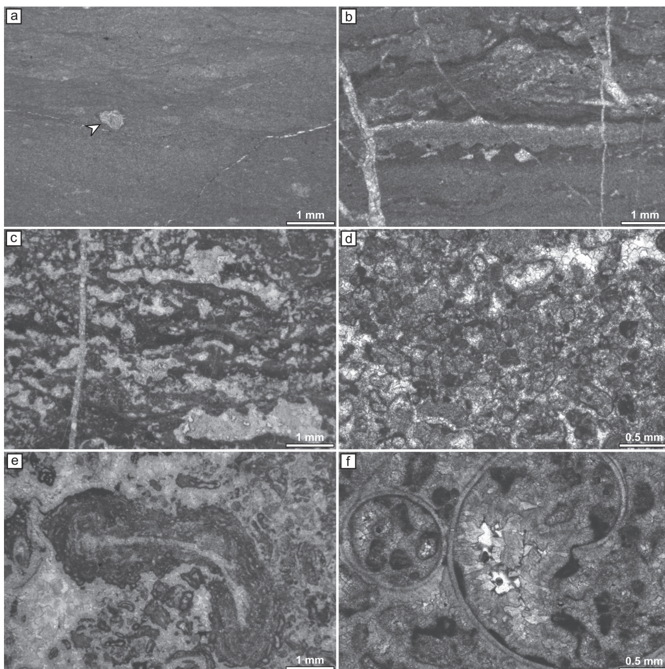
Figure 8. Microfacies of the Velika planina member (upper part), section VP3. a) Bioturbated mudstone with sparse bioclasts. Arrowhead points at the undetermined shell. Thin section 1509. b) Microbial laminated mudstone (stromatolite). Thin section 1511. c) Microbially-bound grainstone with fenestral fabric (stromatolite). Thin section 1528. d) Bioclastic-peloid grainstone. Thin section 1517. e) Oncoid floatstone. A large oncoid, formed mostly by sessile foraminifers, floats in bioclastic-intraclastic grainstone. Thin section 1525. f) Peloid-bioclastic grainstone with gastropod shells. Thin section 1529a.
