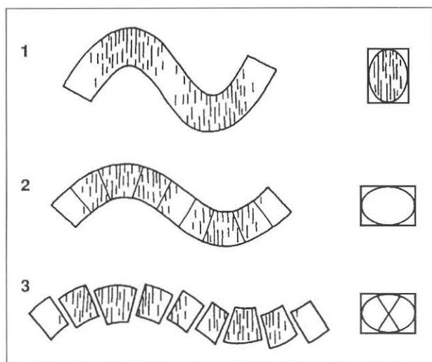
Fig. 7 The sequence of deformation from contraction (1) to extension (2) and gravitational joints (3).
