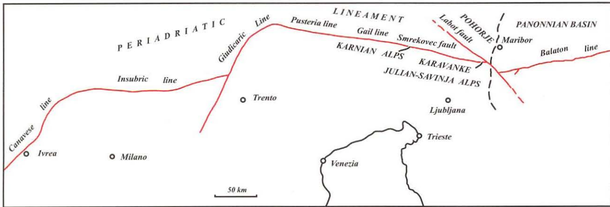
Fig. 1 The geographic position of the Periadriatic Lineament from Iverea zone in Italy to the Pannonian basin in Hungary.
