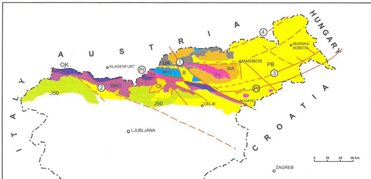
Fig. 3 A generalised tectonic map of the Karavanke Mts. with the boundary tectonic units of the Eastern Alps, Julian-Savinja Alps and Pannonian basin. Legend: JSO) Julian-Savinja units; SKO) South Karavanke overthrust; OK) Olševa-Košuta overthrust; PL) Periadriatic lineament; ZPL) Zone of Periadriatic lineament; NKO) North Karavanke overthrust; MA) Middle Austroalpine; UA) Upper Austroalpine; T) Tonalite of Pohorje; B) Neogene basins; PB) Pannonian basin; 1) Lavantal fault; 2) Sava fault; 3) Ljutomer fault; 4) Raba fault.
