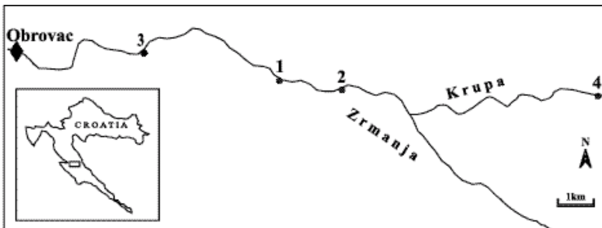
Fig. 1 Location map of the Zrmanja river canyon showing an expanded view of the study area (waterfalls: 1 - Berberi buk, 2 - Ogari buk, 3 - Jankovića buk; cascade: 4 - Krupa). Obrovac marks a downstream direction.
