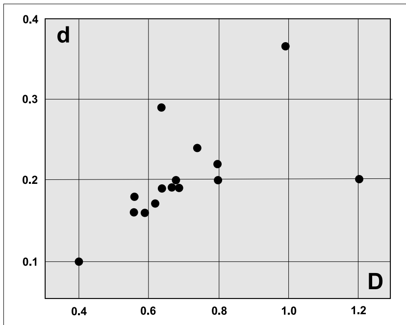
Fig. 3 Neogyroporella? gawlicki n.sp.: outer diameter of the thallus against the inner diameter of the thallus (d). The parameters d and D are well correlated except the value indicated by DYA (1992 – D = 1.2 mm).
