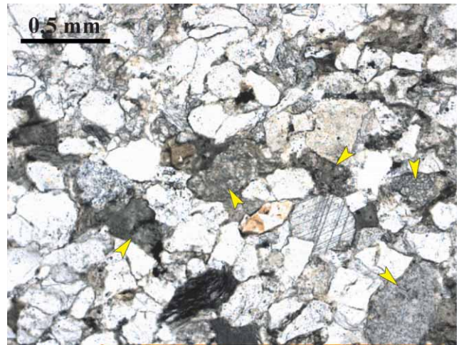
Figure 9: Devitrified volcanic particles in the sandstone showing faint porphyritic structure (arrows) and altered feldspars. Stained with Alizarin and K-ferricyanide. Microphotograph; plane polarised light.
