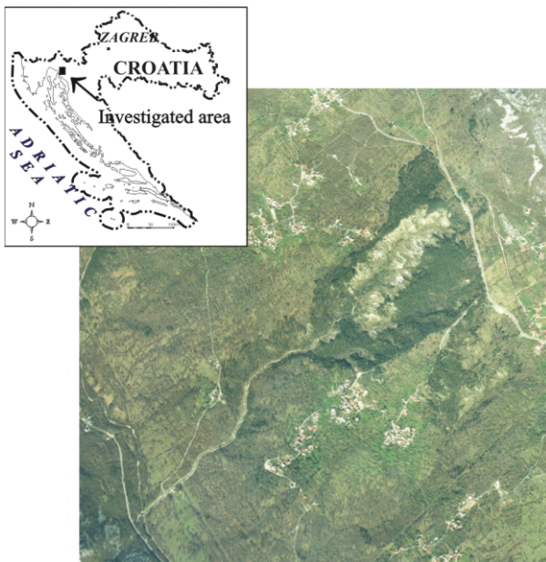
Figure 1: Location of investigated area with air photograph of Vinodol Valley and Slani Potok catchment area (light gray).
