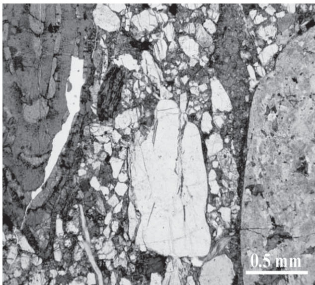
Figure 10: Microphotograph of biocalcirudite ('nummulite breccia'). Note abundance of siliciclastic particles and a large lithic fragment on the right, clearly showing porphyritic structure, with plagioclase fenocrysts and altered microcrystalline quartz/chlorite matrix. Stained with Alizarin and K-ferricyanide. Plane polarized light.
