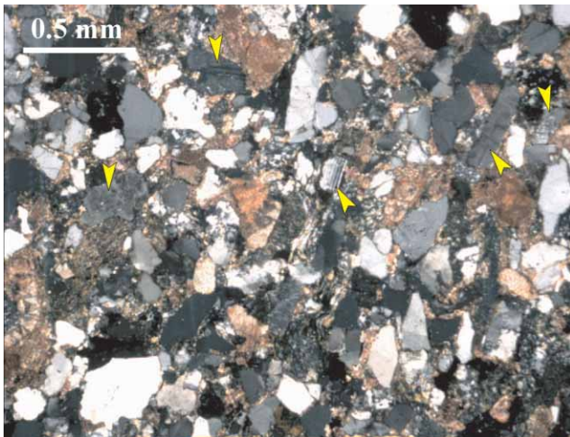
Figure 8: Composition of sandstone. Note prevalence of siliciclastic material (lithic particles and feldspars are marked by arrow). Stained with Alizarin and K-ferricyanide. Microphotograph; crossed nicols.
