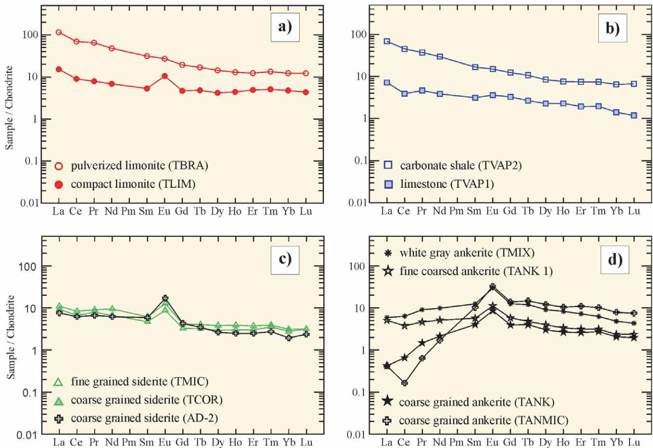
Figure 20: Plot of rare-earth elements normalized to C1 chondrites (SUN & McDONOUGH, 1989) in: a) compact and pulverized limonite; b) limestone and carbonate shale; c) siderite; d) ankerite.
