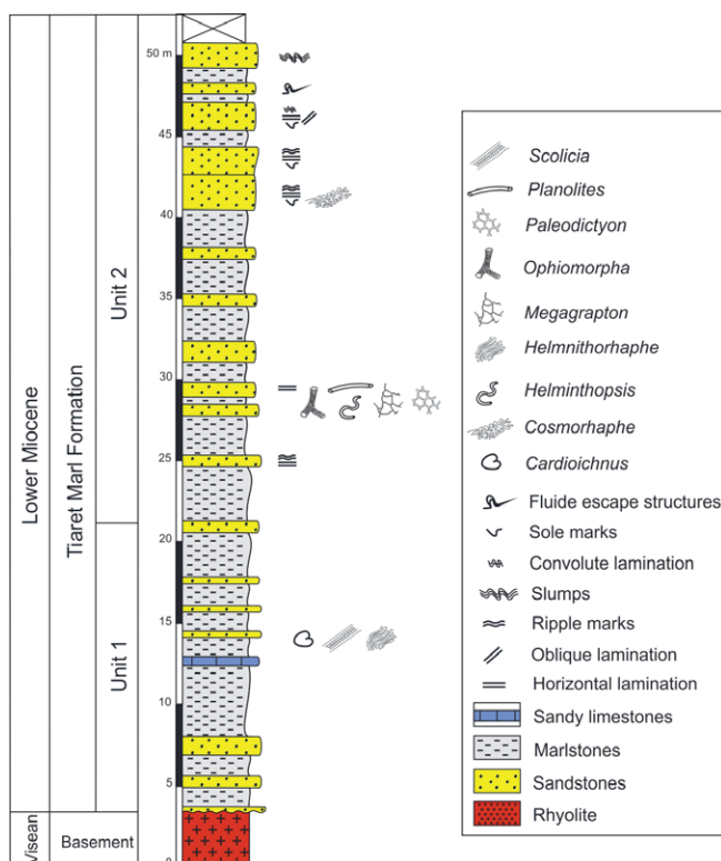
Figure 2. The stratigraphic succession and vertical distribution of trace fossils of the lower Miocene Tiaret Marls Formation in the Sidi Ali Mellal section.
