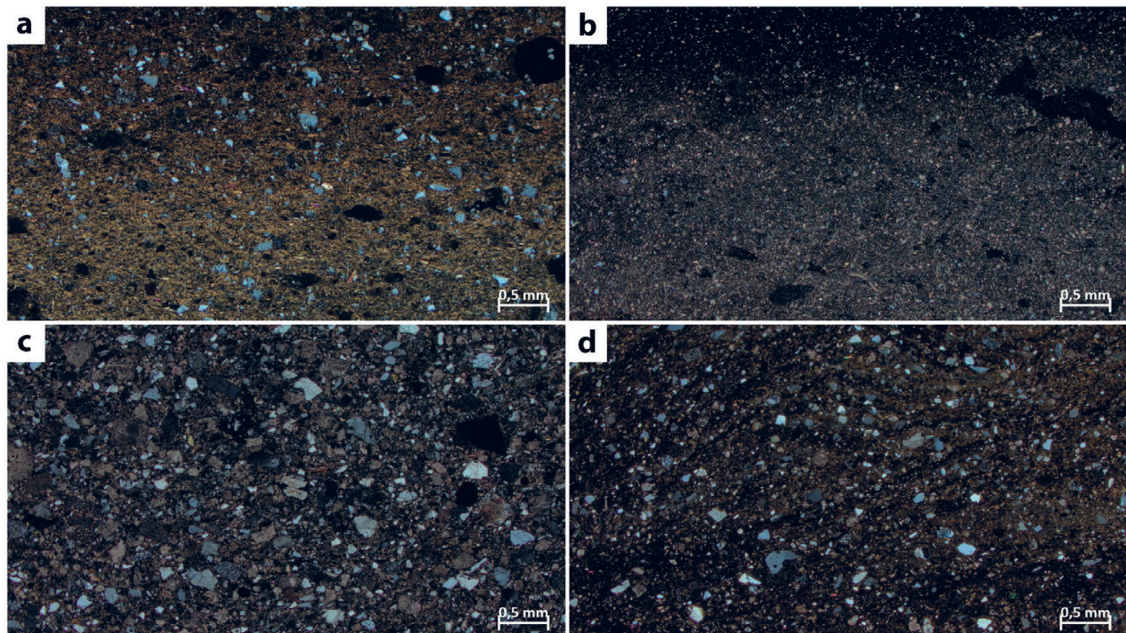
Figure 4. Thin section photomicrographs of fired clay briquettes; (a) sample 102, (b) sample 105, (c) sample 107 and (d) sample 108.
